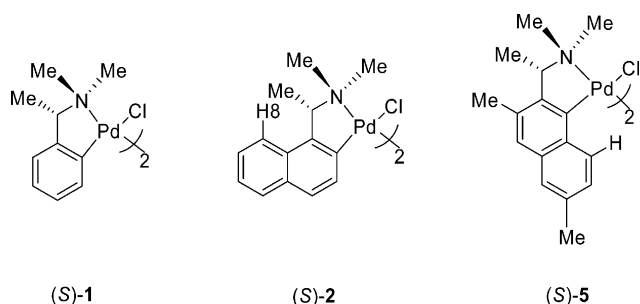
Figure 1. Molecular design for complexes ( S )-1, ( S )-2, and ( S )-5.
