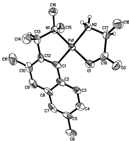
Figure 6. Molecular structure of (cis\text{-}N,N)\text{-(}R_C,S_C\text{)}\text{-13} .
