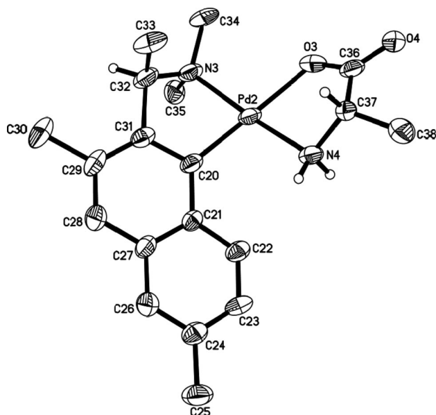
Figure 5. Molecular structure of (trans\text{-}N,N)\text{-(}R_C,S_C\text{)}\text{-13} .
