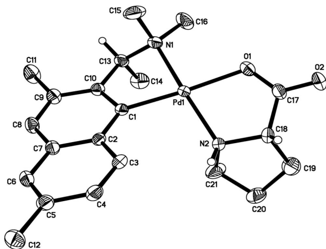
Figure 4. Molecular structure of (S_C, S_C, S_N)\text{-12} .
