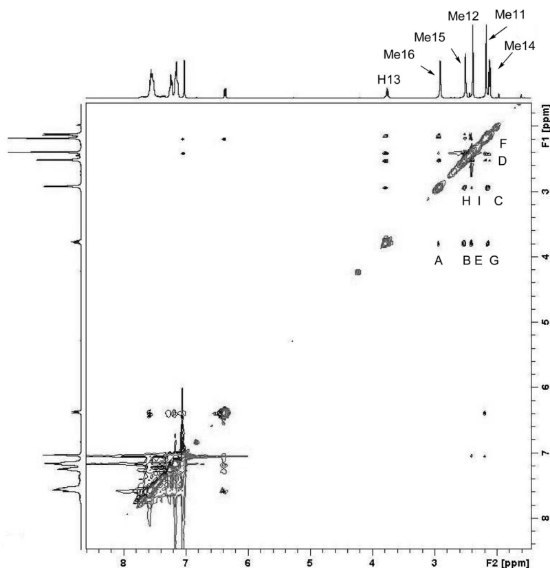
Figure 3. 2D ^1\text{H} – ^1\text{H} ROESY NMR spectrum of (\pm) - 11 in \text{CDCl}_3 .
