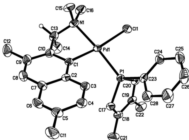
Figure 8. Molecular structure of (S)-14.
