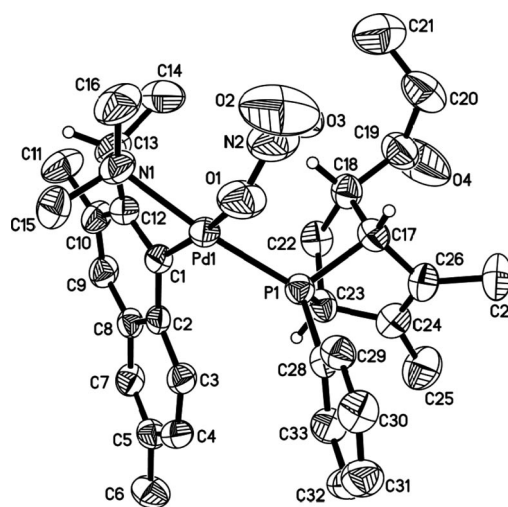
Figure 9. Molecular structure of ( S C , R P )- 16 .
