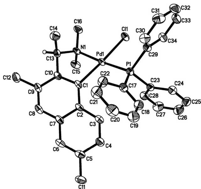
Figure 2. Molecular structure of (±)- 11 .
