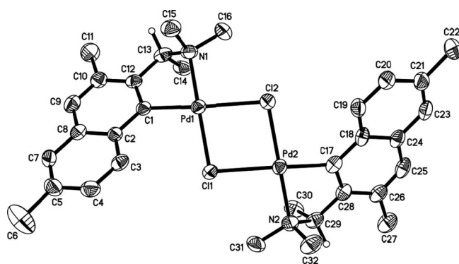
Figure 7. Molecular structure of (S)-5.
